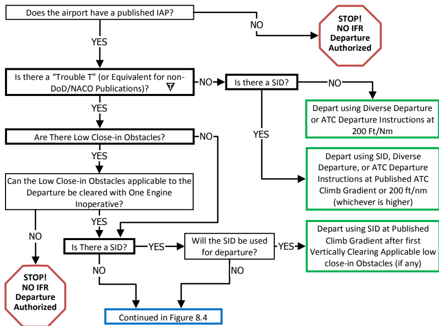
Figure 8.3. Normal IFR Departure Options Decision Tree (Page 1)
